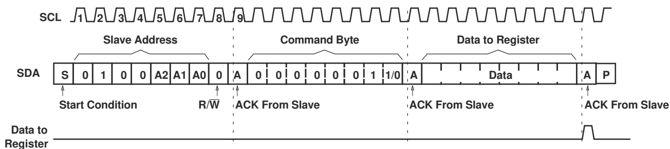
Figure 8-9. Write To Configuration Or Polarity Inversion Registers
