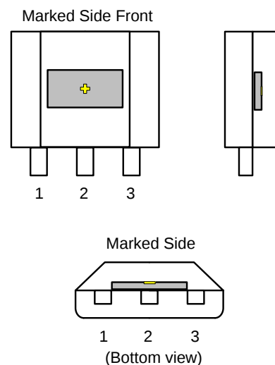
Figure 19. TO-92 (LPG) Package
