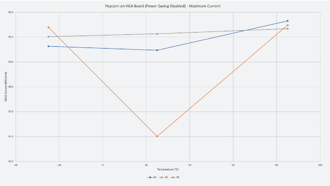
Figure 10. Popcorn running on the VGA board (maximum current) with power saving disabled (GPIO23 pulled high)
