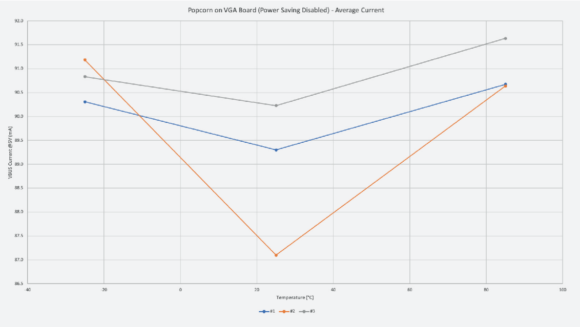
Figure 9. Popcorn running on the VGA board (average current) with power saving disabled (GPIO23 pulled high)
